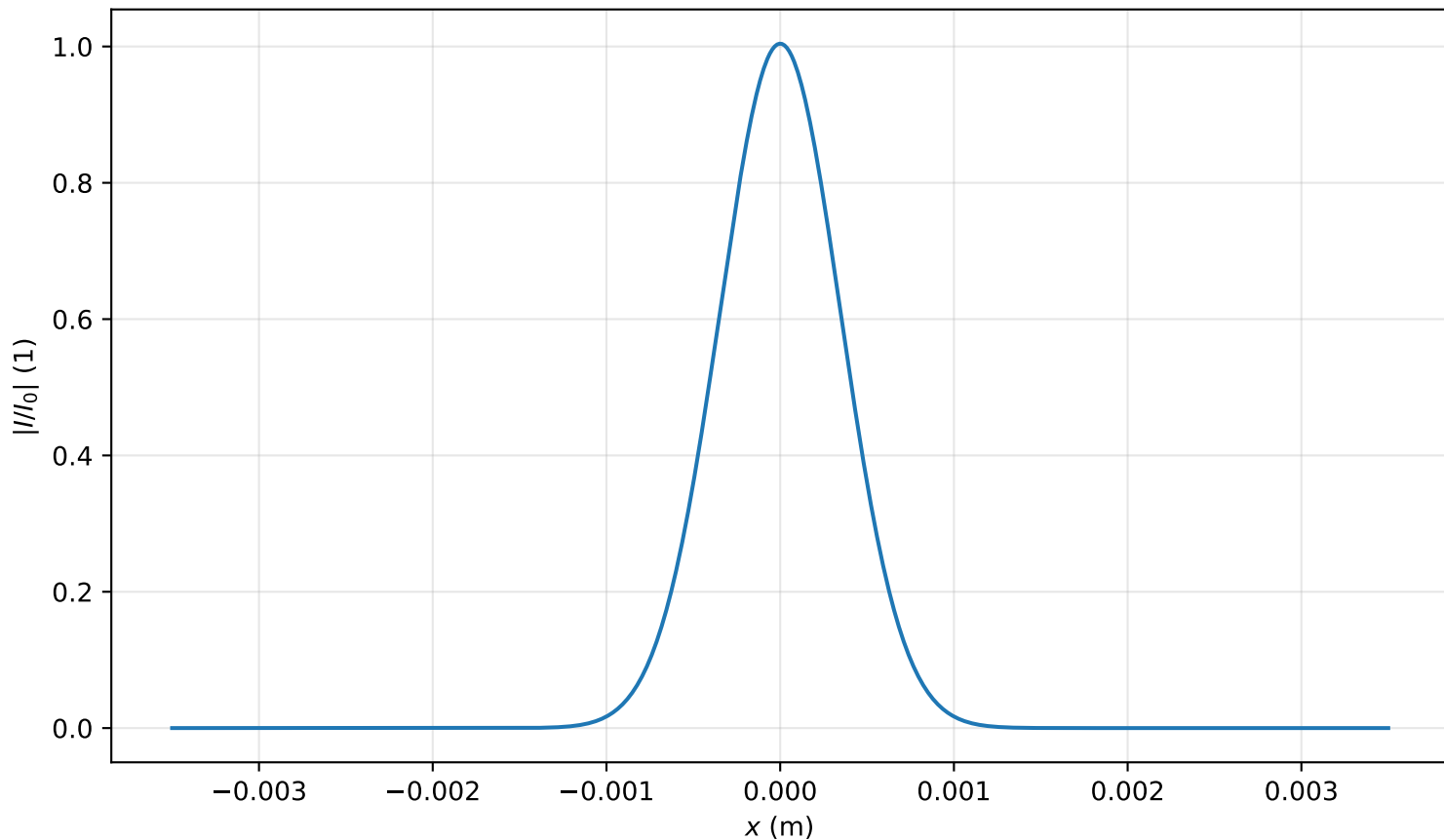
Intensity profile I(x, y = 0, z = 0.080m)/I_0 , P_{in}=0.9P_{cr} , artificial time
